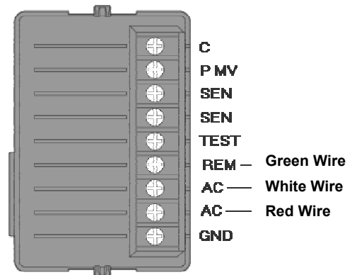
Simple Three Wire Installation
