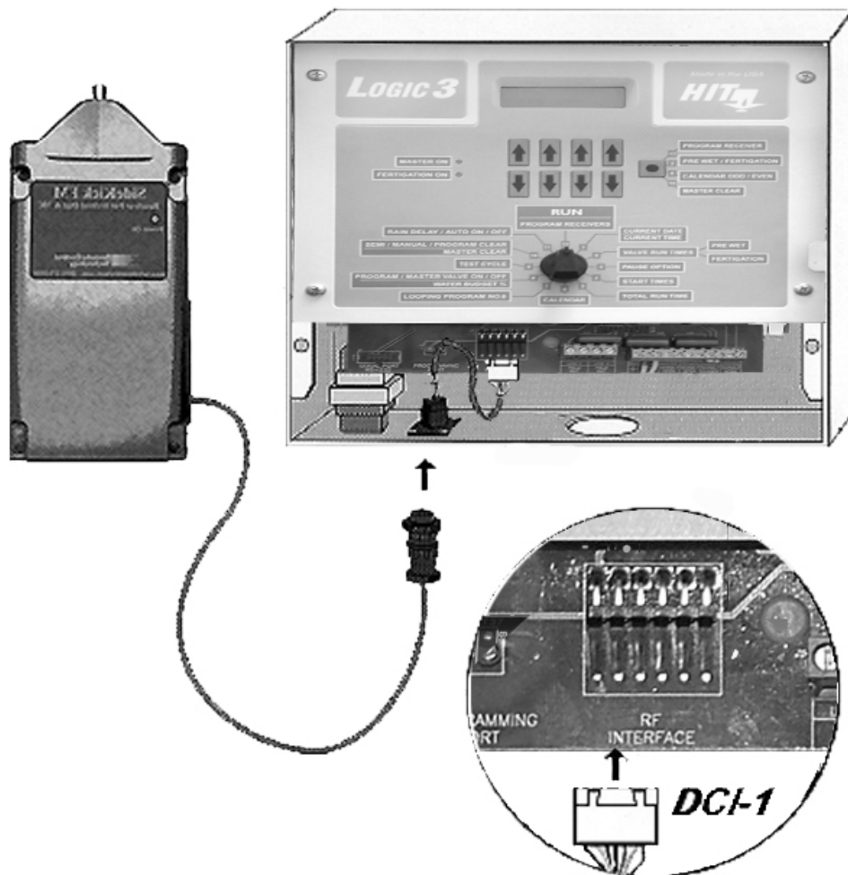
DCI-1 Cable and Sidekick Receiver installation
