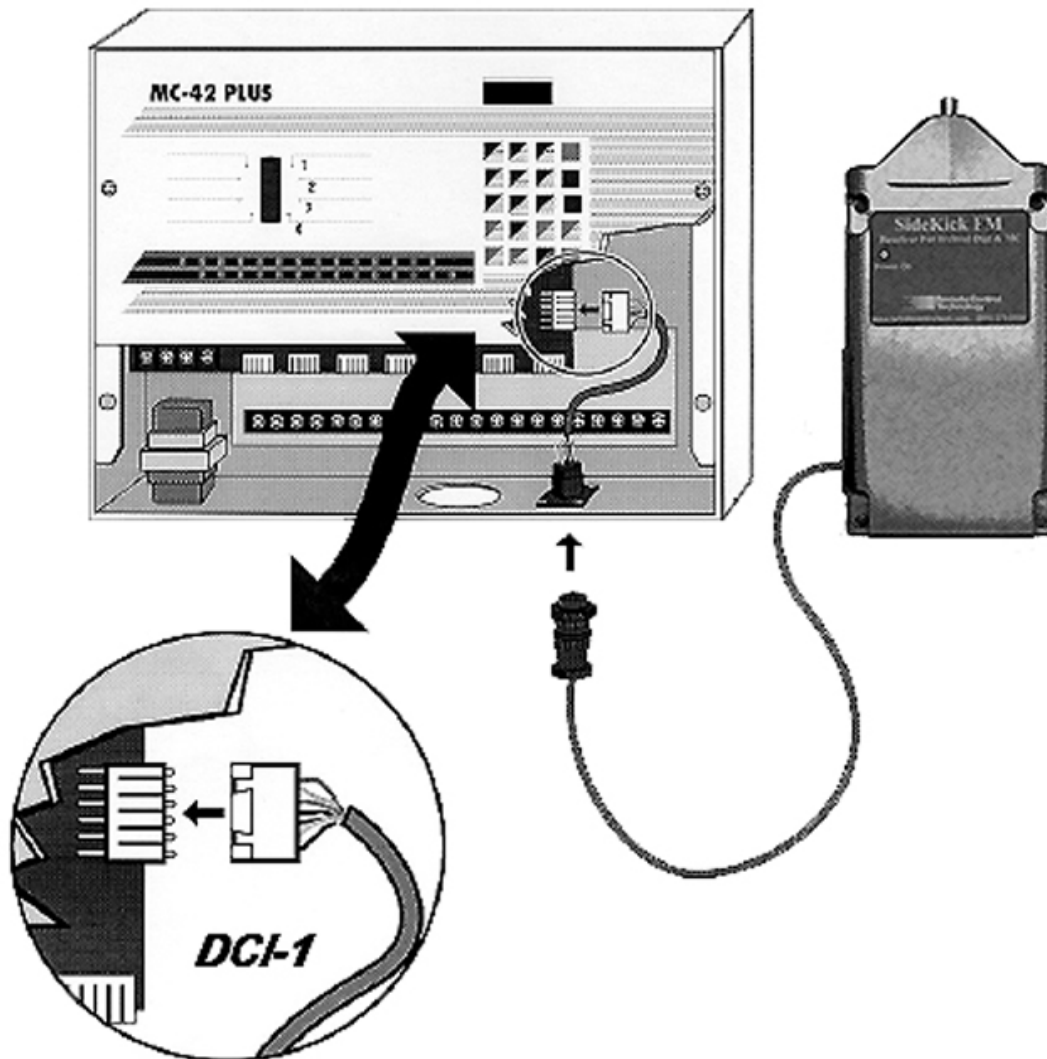
DCI-1 Cable and Sidekick Receiver installation
