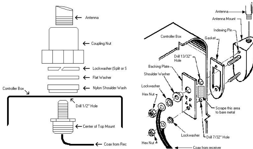
Top Mount Antenna Diagram Side Mount Antenna Diagram
